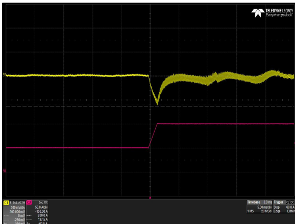
Figure 9: DS1200HE-3-002 Transient Response - V_O Deviation 50% to 100% load change 1A/uS slew rate V_{in} = 230Vac Ch 1: V_O Ch 2: I_O
