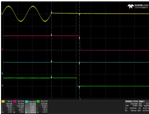
Figure 3: DS1200HE-3-002 Hold-up Time Vin = 90Vac Load: I O = 83.3A I SB = 4A (5V) Ch 1: AC Mains Ch 2: V O Ch 3: V SB Ch 4: Pwr_GOOD
