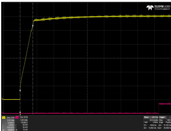
Figure 5: DS1200HE-3-002 Output Voltage Startup Characteristic Vin = 90Vac Load: I O = 83.3A I SB = 4A (5V) Ch 1: V O Ch 2: Pwr_GOOD
