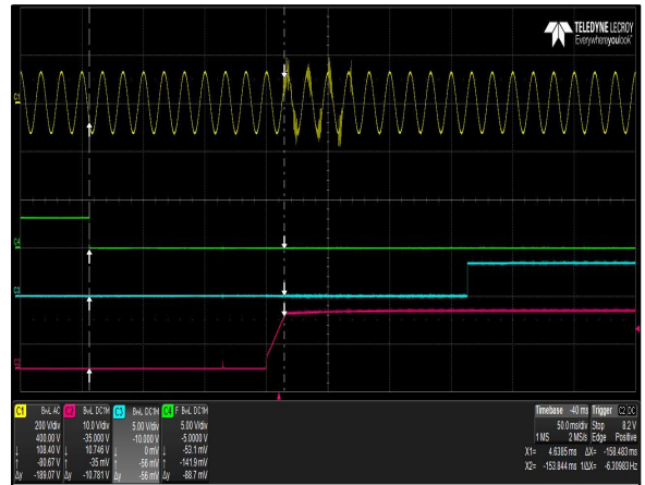
Figure 2: DS1200HE-3-002 Turn-On Delay via PS_ON Vin = 90Vac Load: I O = 62.5A I SB = 4A (5V) Ch 1: AC Mains Ch 2: V O Ch 3: Pwr_GOOD Ch 4: PS_ON
