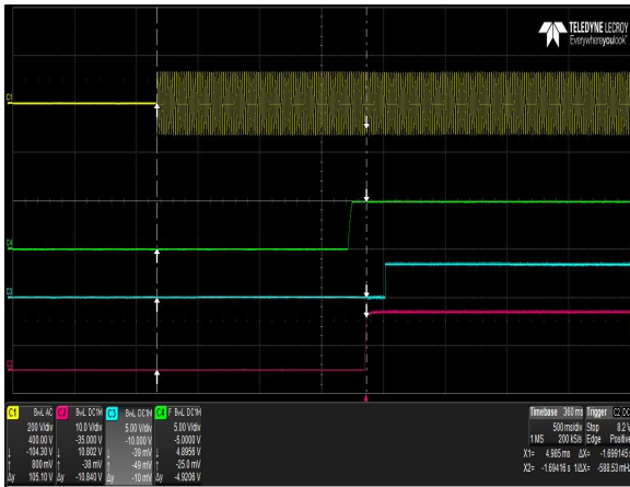
Figure 1: DS1200HE-3-002 Turn-On Delay via AC Mains Vin = 90Vac Load: I O = 83.3A I SB = 4A (5V) Ch 1: AC Mains Ch 2: V O Ch 3: Pwr_GOOD Ch 4: V SB
