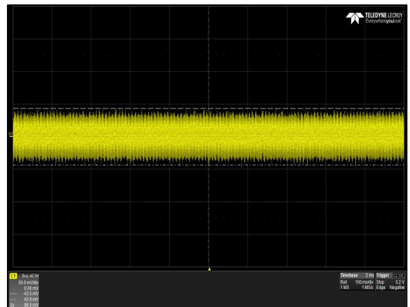
Figure 6: DS1200HE-3-002 Ripple and Noise Measurement Vin = 115Vac Load: I O = 83.3A I SB = 4A (5V) Ch 1: V O
