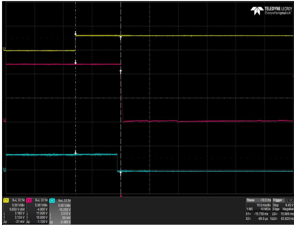
Figure 7: DS1200HE-3-002 Turn Off Characteristic via PS_ON Load: I_O = 81.7A I_{SB} = 4A (5V) Ch 1: PS_ON Ch 2: V_O Ch 3: Pwr_GOOD
