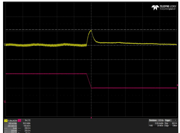
Figure 10: DS1200HE-3-002 Transient Response - V_O Deviation 100% to 50% load change 1A/uS slew rate V_{in} = 230Vac Ch 1: V_O Ch 2: I_O
