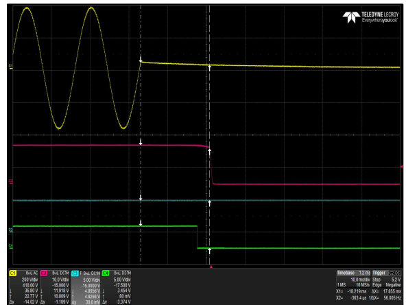
Figure 4: DS1200HE-3-002 Hold-up Time Vin = 264Vac Load: I O = 100A I SB = 4A (5V) Ch 1: AC Mains Ch 2: V O Ch 3: V SB Ch 4: Pwr_GOOD
