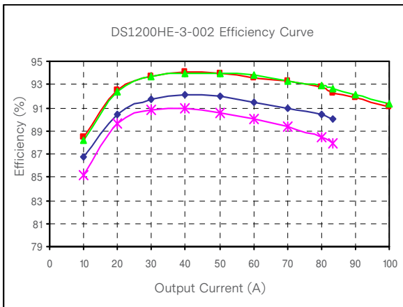
Figure 11: DS1200HE-3-002 Efficiency Curve @ 25°C Loading: I_{o\_main} = 10\%I_{o\_max} increment to 100A, I_{SB} = 0A (5V)
