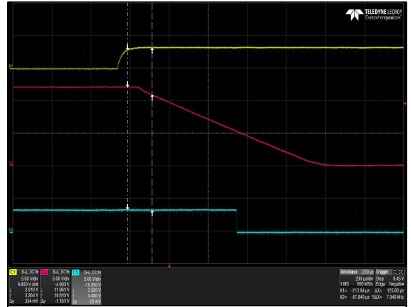
Figure 8: DS1200HE-3-002 Turn Off Characteristic via PS_INHIBIT Load: I_O = 81.7A I_{SB} = 4A (5V) Ch 1: PS_INHIBIT Ch 2: V_O Ch 3: Pwr_GOOD
