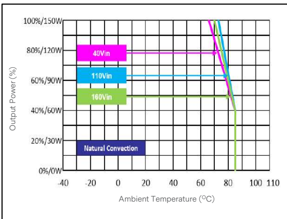
Figure 44: ERM6H100 Derating Curve with 3U iron back-plate (Dimension 482X133.5X1.6mm) Vin = 40 to 160 Vdc Load: Io = 0 to 6.25 A
