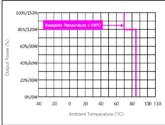
Figure 18: ERM12B100 Derating Curve without Heatsink Vin = 110Vdc Load: Io = 0 to 12.5 A
