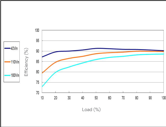
Figure 34: ERM6H100 Efficiency Versus Output Current Curve Vin = 40 to 160 Vdc Load: Io = 0 to 6.25 A
