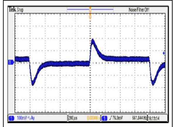
Figure 26: ERM10C100 Transient Response Vin = 110Vdc Load: Io = 100% to 75% load change Ch 1: Vo
