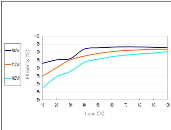
Figure 12: ERM12B100 Efficiency Versus Output Current Curve Vin = 40 to 160 Vdc Load: Io = 0 to 12.5 A
