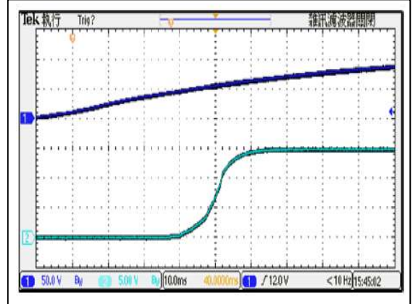
Figure 28: ERM10C100 Output Voltage Startup Characteristic by Vin Vin = 110Vdc Load: Io = 10A Ch 1: Vin Ch 2: Vo
