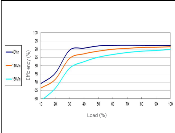
Figure 1: ERM30A100 Efficiency Versus Output Current Curve Vin = 40 to 160 Vdc Load: Io = 0 to 27 A
