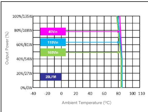
Figure 9: ERM30A100 Derating Curve with 3U iron back-plate (Dimension 482X133.5X1.6mm) Vin = 40 to 160 Vdc Load: Io = 0 to 27 A
