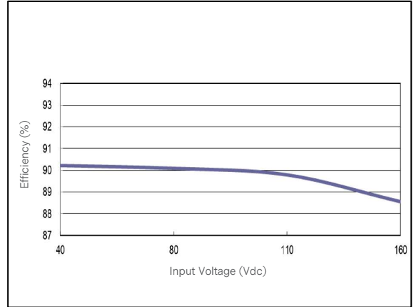
Figure 35: ERM6H100 Efficiency Versus Input Voltage Curve Vin = 40 to 160Vdc Load: Io = 0 to 6.25 A
