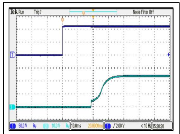
Figure 39: ERM6H100 Output Voltage Startup Characteristic by Vin Vin = 110Vdc Load: Io = 6.25A Ch 1: Vin Ch 2: Vo
