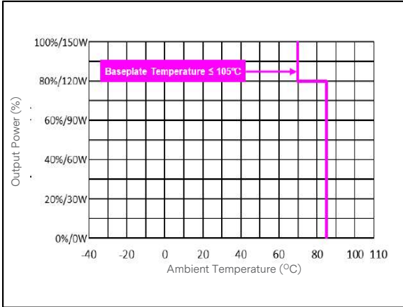
Figure 40: ERM6H100 Derating Curve without Heatsink Vin = 110Vdc Load: Io = 0 to 6.25 A
