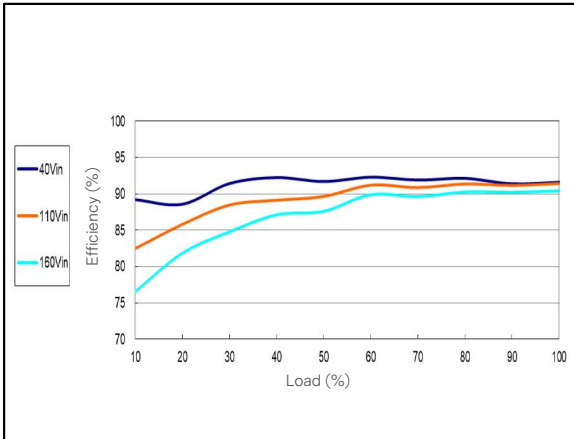
Figure 45: ERM02U100 Efficiency Versus Output Current Curve Vin = 40 to 160 Vdc Load: Io = 0 to 2.78 A
