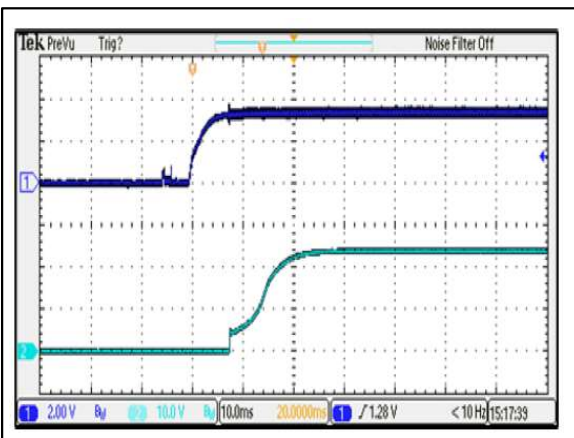
Figure 38: ERM6H100 Output Voltage Startup Characteristic by On/Off Vin = 110Vdc Load: Io = 6.25A Ch 1: Remote On/Off Ch 2: Vo
