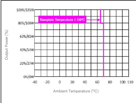
Figure 7: ERM30A100 Derating Curve without Heatsink Vin = 110Vdc Load: Io = 0 to 27 A
