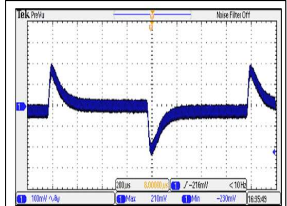
Figure 15: ERM12B100 Transient Response Vin = 50Vdc Load: Io = 100% to 75% load change Ch 1: Vo
