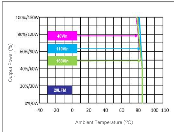
Figure 20: ERM12B100 Derating Curve with 3U iron back-plate (Dimension 482X133.5X1.6mm) Vin = 40 to 160 Vdc Load: Io = 0 to 12.5 A
