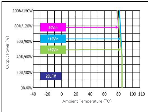
Figure 31: ERM10C100 Derating Curve with 3U iron back-plate (Dimension 482X133.5X1.6mm) Vin = 40 to 160 Vdc Load: Io = 0 to 10 A
