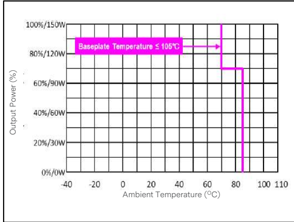
Figure 29: ERM10C100 Derating Curve without Heatsink Vin = 110Vdc Load: Io = 0 to 10 A
