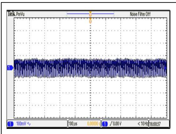
Figure 47: ERM02U100 Typical Output Ripple and Noise Vin = 110Vdc Load: Io = 2.78A Ch 1: Vo
