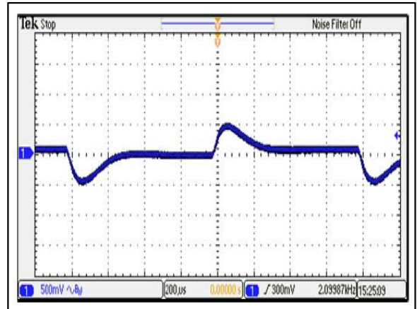
Figure 37: ERM6H100 Transient Response Vin = 110Vdc Load: Io = 100% to 75% load change Ch 1: Vo
