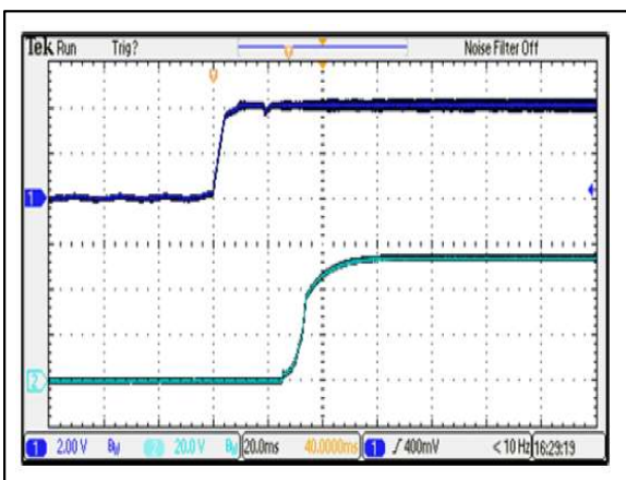
Figure 49: ERM02U100 Output Voltage Startup Characteristic by On/Off Vin = 110Vdc Load: Io = 2.78A Ch 1: Remote On/Off Ch 2: Vo
