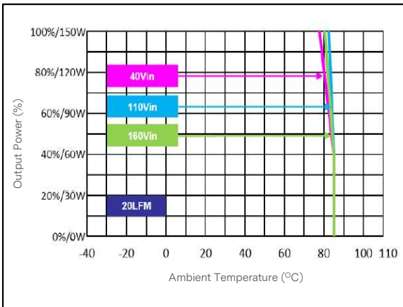
Figure 42: ERM6H100 Derating Curve with 3U iron back-plate (Dimension 482X133.5X1.6mm) Vin = 40 to 160 Vdc Load: Io = 0 to 6.25 A
