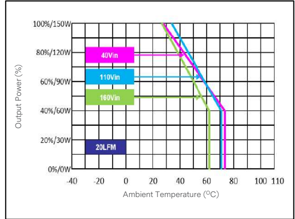
Figure 41: ERM6H100 Derating Curve with HS7 Heatsink Vin = 40 to 160 Vdc Load: Io = 0 to 6.25 A
