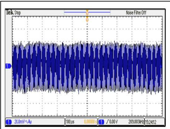
Figure 36: ERM6H100 Typical Output Ripple and Noise Vin = 110Vdc Load: Io = 6.25A Ch 1: Vo
