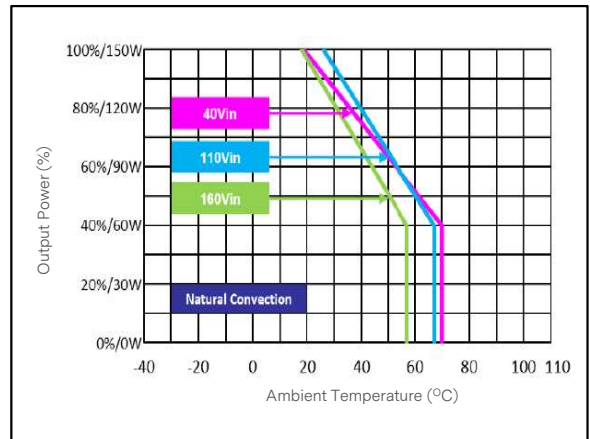
Figure 43: ERM6H100 Derating Curve with HS7 Heatsink Vin = 40 to 160 Vdc Load: Io = 0 to 6.25 A
