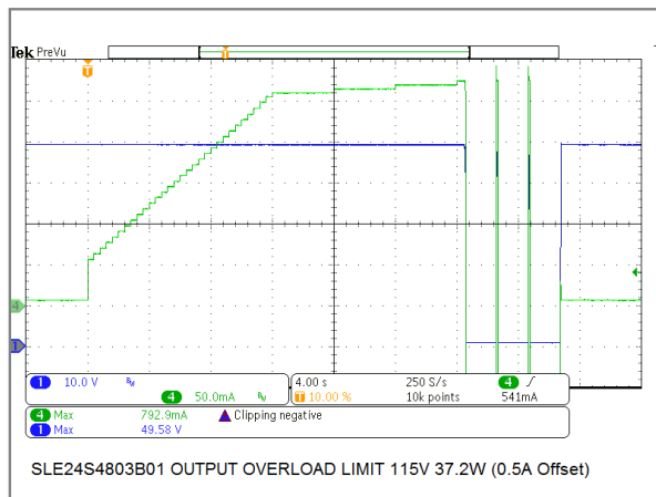
24W/48V Model Output Overload Protection
