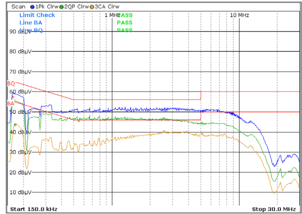
24W/24V Model _ Neutral 120V/60Hz 100% 24V@1.0A
