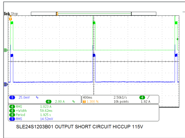
24W/12V Model Output Short Circuit Hiccup Mode
