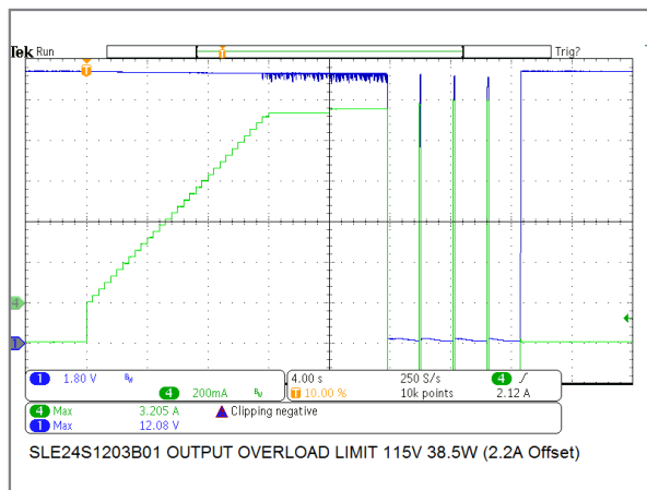
24W/12V Model Output Overload Protection
