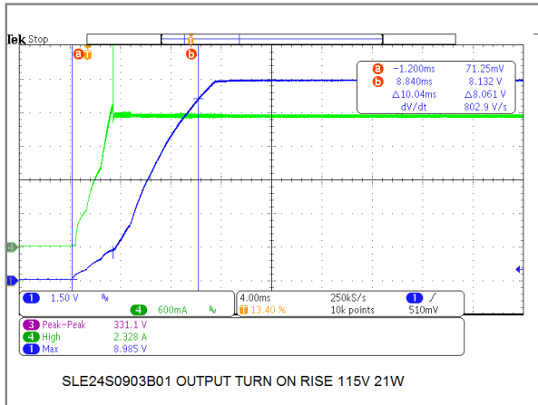
24W/9V Model Output Turn-On Rise Time
