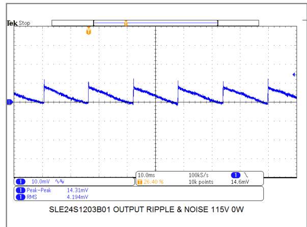
24W/12V Model Output Ripple & Noise at No Load
