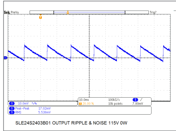
24W/24V Model Output Ripple & Noise at No Load
