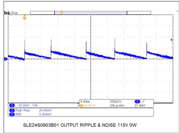
24W/9V Model Output Ripple & Noise at No Load
