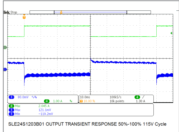
24W/12V Model Transient Response
