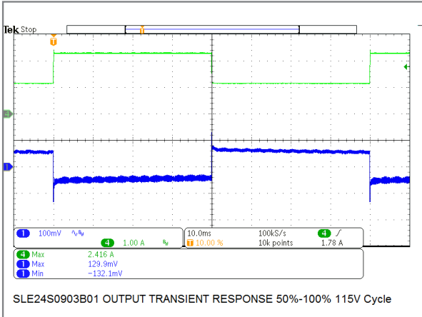
24W/9V Model Transient Response
