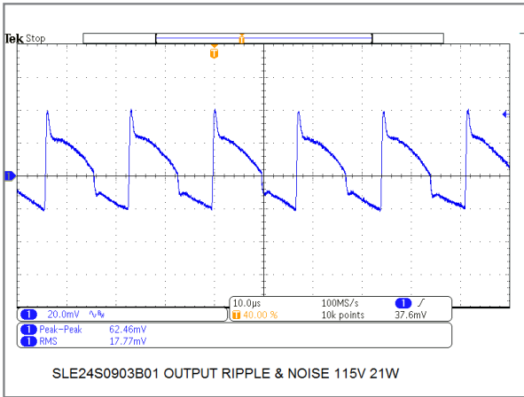
24W/9V Model Output Ripple & Noise at Full Load
