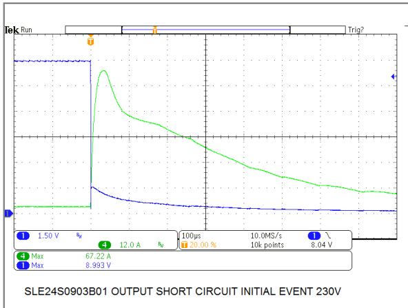
24W/9V Model Output Short Circuit Initial Event
