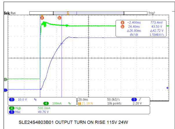
24W/48V Model Output Turn-On Rise Time
