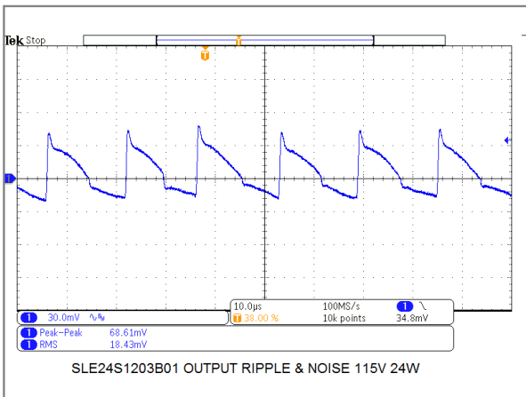
24W/12V Model Output Ripple & Noise at Full Load
