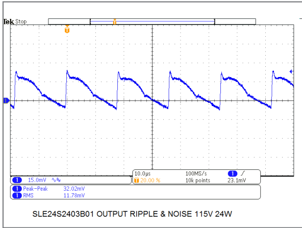
24W/24V Model Output Ripple & Noise at Full Load
