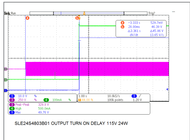
24W/48V Model Turn-On Delay Time
