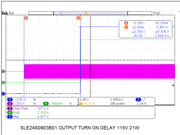
24W/9V Model Turn-On Delay Time
