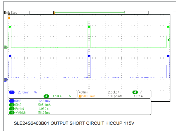
24W/24V Model Output Short Circuit Hiccup Mode
