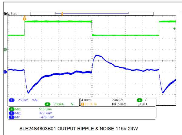
24W/48V Model Transient Response
