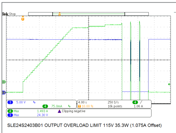
24W/24V Model Output Overload Protection
