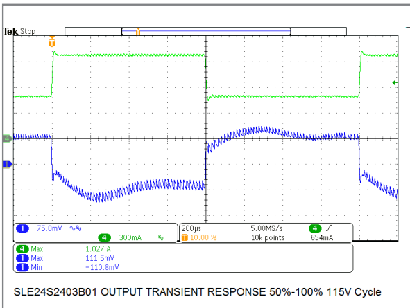
24W/24V Model Transient Response
