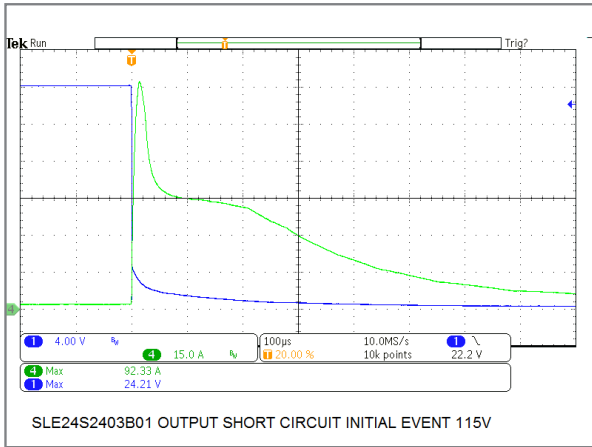
24W/24V Model Output Short Circuit Initial Event
