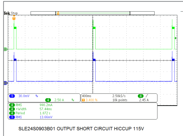
24W/9V Model Output Short Circuit Hiccup Mode
