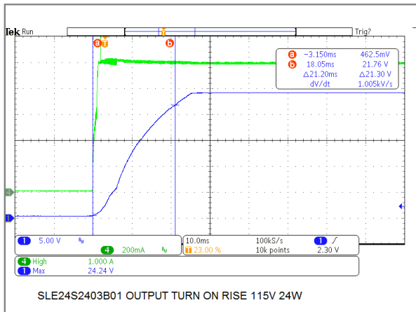
24W/24V Model Output Turn-On Rise Time
