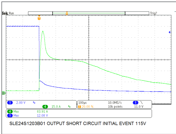
24W/12V Model Output Short Circuit Initial Event
