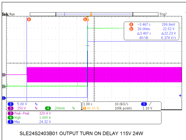
24W/24V Model Turn-On Delay Time
