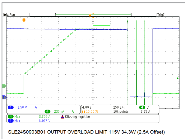
24W/9V Model Output Overload Protection
