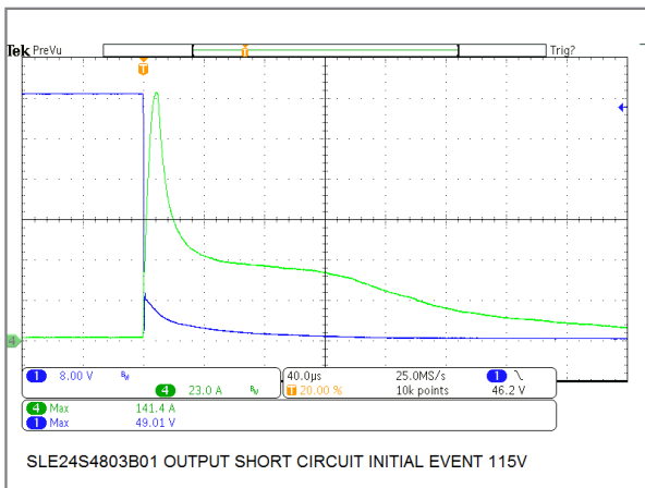
24W/48V Model Output Short Circuit Initial Event
