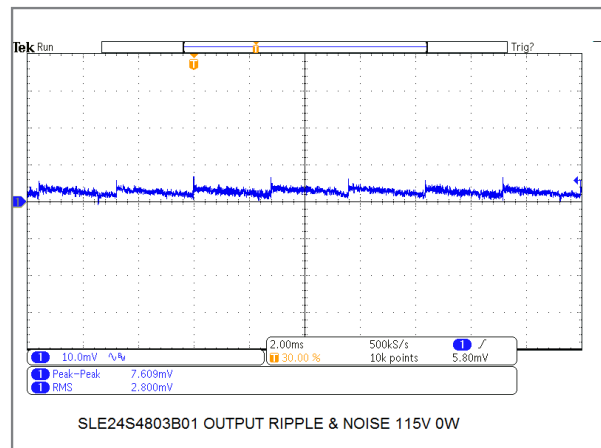
24W/48V Model Output Ripple & Noise at No Load
