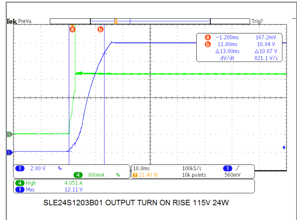
24W/12V Model Output Turn-On Rise Time
