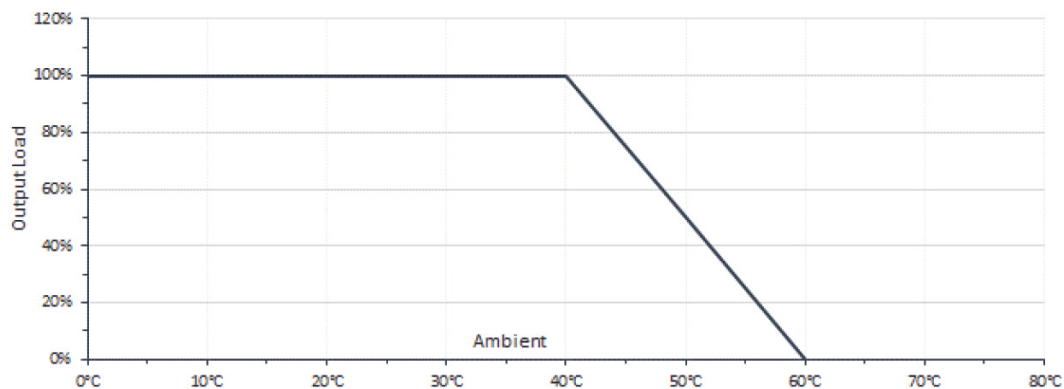
Figure 2: SLE24 family derating curve
