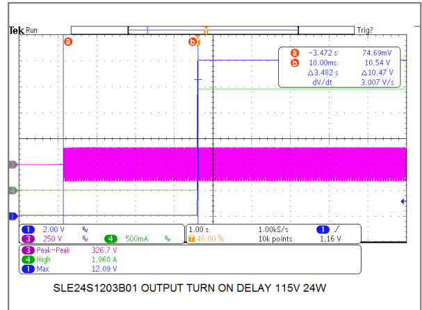
24W/12V Model Turn-On Delay Time
