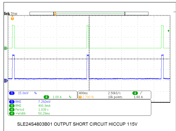
24W/48V Model Output Short Circuit Hiccup Mode
