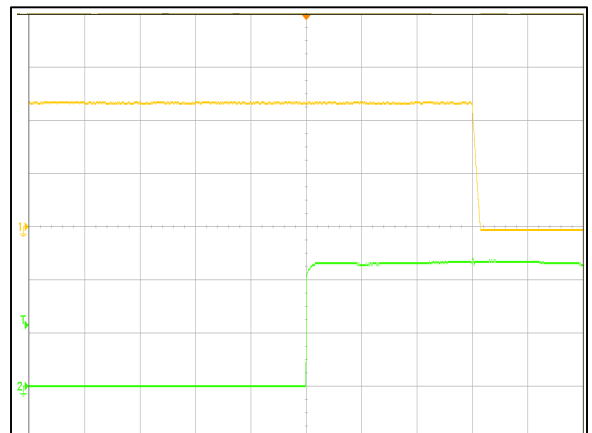
Figure 6: AVO200-48S12-6L Remote OFF Waveform (20mS/div) Vin = 36Vdc Load: Io = 16.7A Ch 1: Vo (5V/div) Ch 2: Remote OFF (2V/div)
