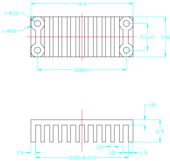
Figure 24 Temperature test point & heat sink mechanical diagram
