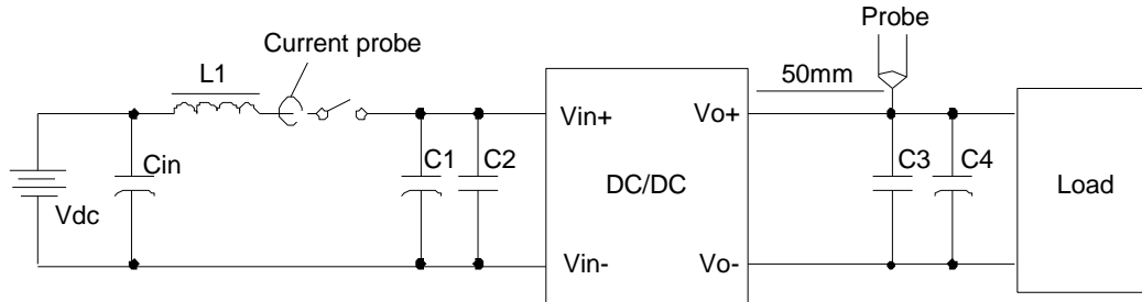
Figure 30 Input ripple &amp; output ripple &amp; noise test configuration
