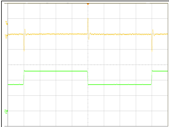
Figure 16: AVO200-48S12B-6L Transient Response (1mS/div) 50%~75%~50% load change, 0.1A/uS slew rate, Vin = 48Vdc Ch 1: Vo (50mV/div) Ch 2: Io (5A/div)
