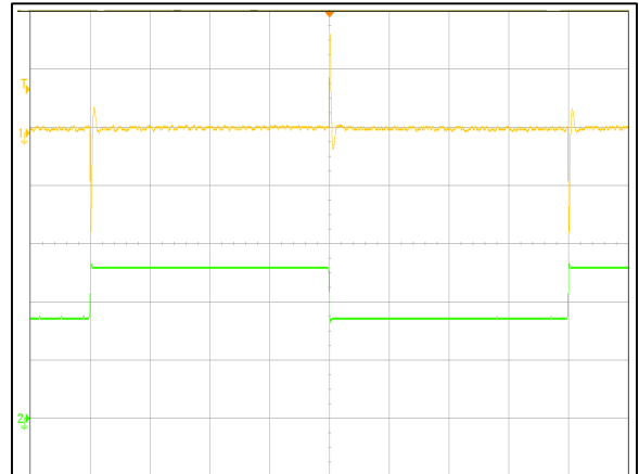
Figure 8: AVO200-48S12-6L Transient Response (1mS/div) 50%~75%~50% load change, 1A/uS slew rate, Vin = 48Vdc Ch 1: Vo (50mV/div) Ch 2: Io (5A/div)
