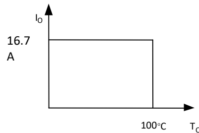
Figure 23 Output power derating curve, T c : temperature test point on baseplate, see Figure 15
