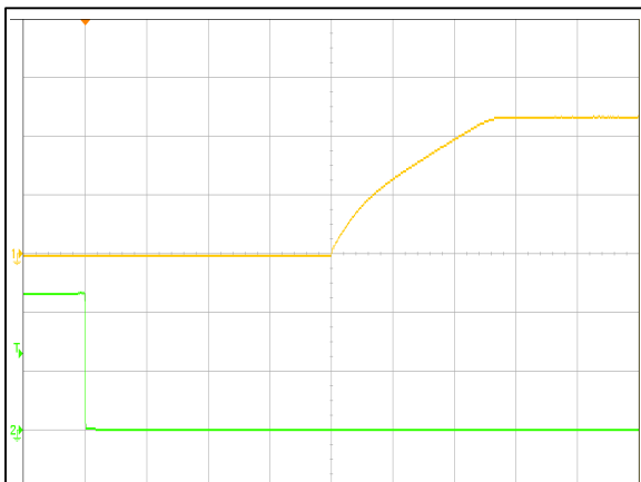
Figure 14: AVO200-48S12B-6L Remote ON Waveform (5mS/div) Vin = 36Vdc Load: Io = 16.7A Ch 1: Vo (5V/div) Ch 2: Remote ON (2V/div)
