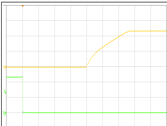
Figure 5: AVO200-48S12-6L Remote ON Waveform (50mS/div) Vin = 36Vdc Load: Io = 16.7A Ch 1: Vo (5V/div) Ch 2: Remote ON (2V/div)
