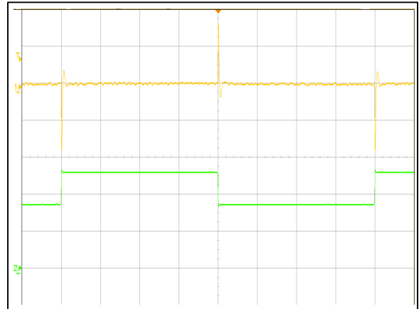
Figure 17: AVO200-48S12B-6L Transient Response (1mS/div) 50%~75%~50% load change, 1A/uS slew rate, Vin = 48Vdc Ch 1: Vo (50mV/div) Ch 2: Io (5A/div)
