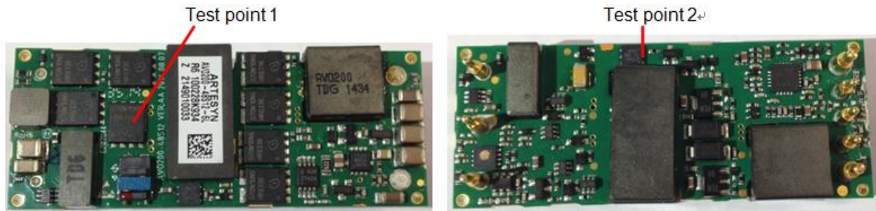
Figure 20 Temperature test point
