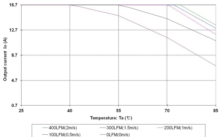
Figure 25 Output power derating, 48Vin, air flowing across the converter (from pin 3 to pin1)
