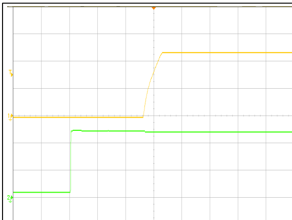
Figure 3: AVO200-48S12-6L Output Voltage Startup Characteristic Vin = 36Vdc Load: Io = 16.7A (2mS/div) Ch 1: Vo (2V/div) Ch 2: Vin (20V/div)
