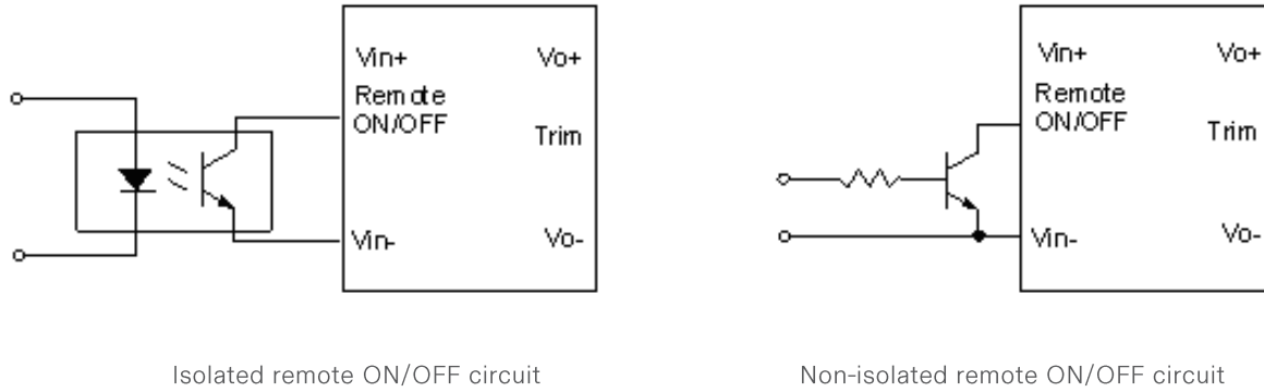
Figure 27 External Remote ON/OFF circuit
