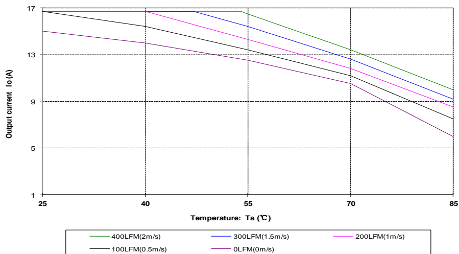
Figure 21 Output power derating, 48Vin, air flowing across the converter from pin 3 to pin 1
