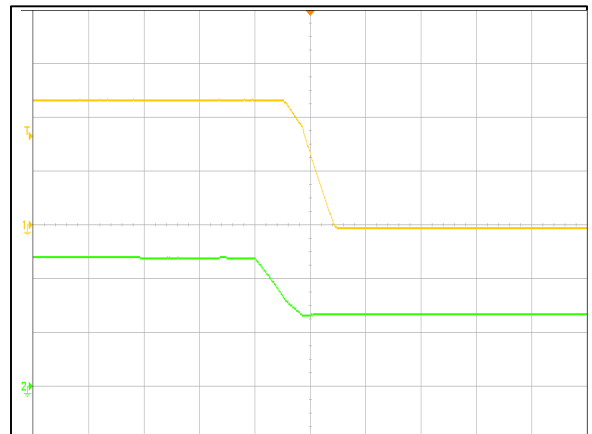
Figure 13: AVO200-48S12B-6L Turn Off Characteristic (1mS/div) Vin = 36Vdc Load: Io = 16.7A Ch 1: Vo (5V/div) Ch 2: Vin (20V/div)
