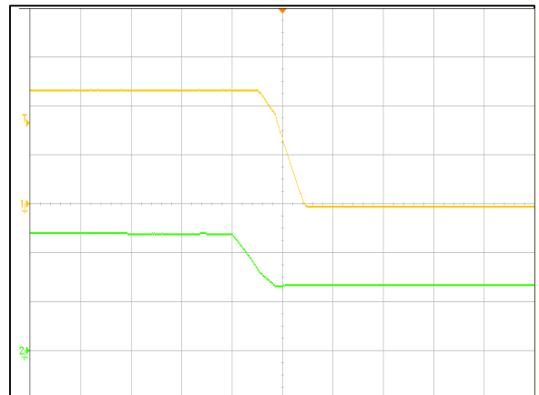
Figure 4: AVO200-48S12-6L Turn Off Characteristic (1mS/div) Vin = 36Vdc Load: Io = 16.7A Ch 1: Vo (2V/div) Ch 2: Vin (20V/div)
