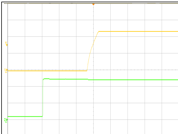
Figure 12: AVO200-48S12B-6L Output Voltage Startup Characteristic Vin = 36Vdc Load: Io = 16.7A (2mS/div) Ch 1: Vo (5V/div) Ch 2: Vin (20V/div)
