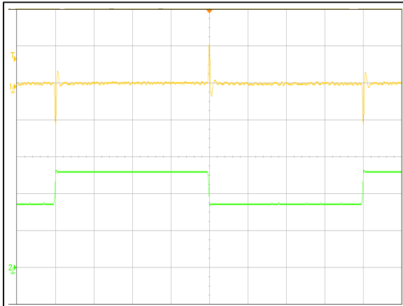
Figure 7: AVO200-48S12-6L Transient Response (1mS/div) 50%~75%~50% load change, 0.1A/uS slew rate, Vin = 48Vdc Ch 1: Vo (50mV/div) Ch 2: Io (5A/div)
